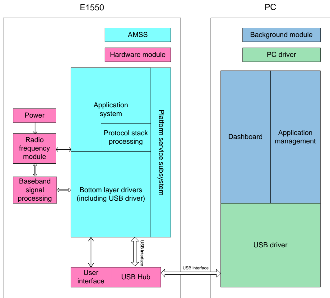
Figure 4-1 System architecture
